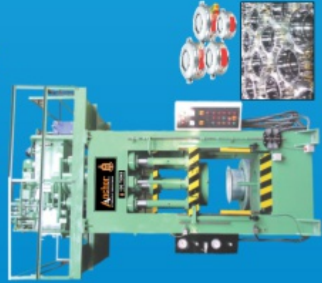
200 TONS BLANK HOLDER TYPE DEEP DRAWING PRESS
